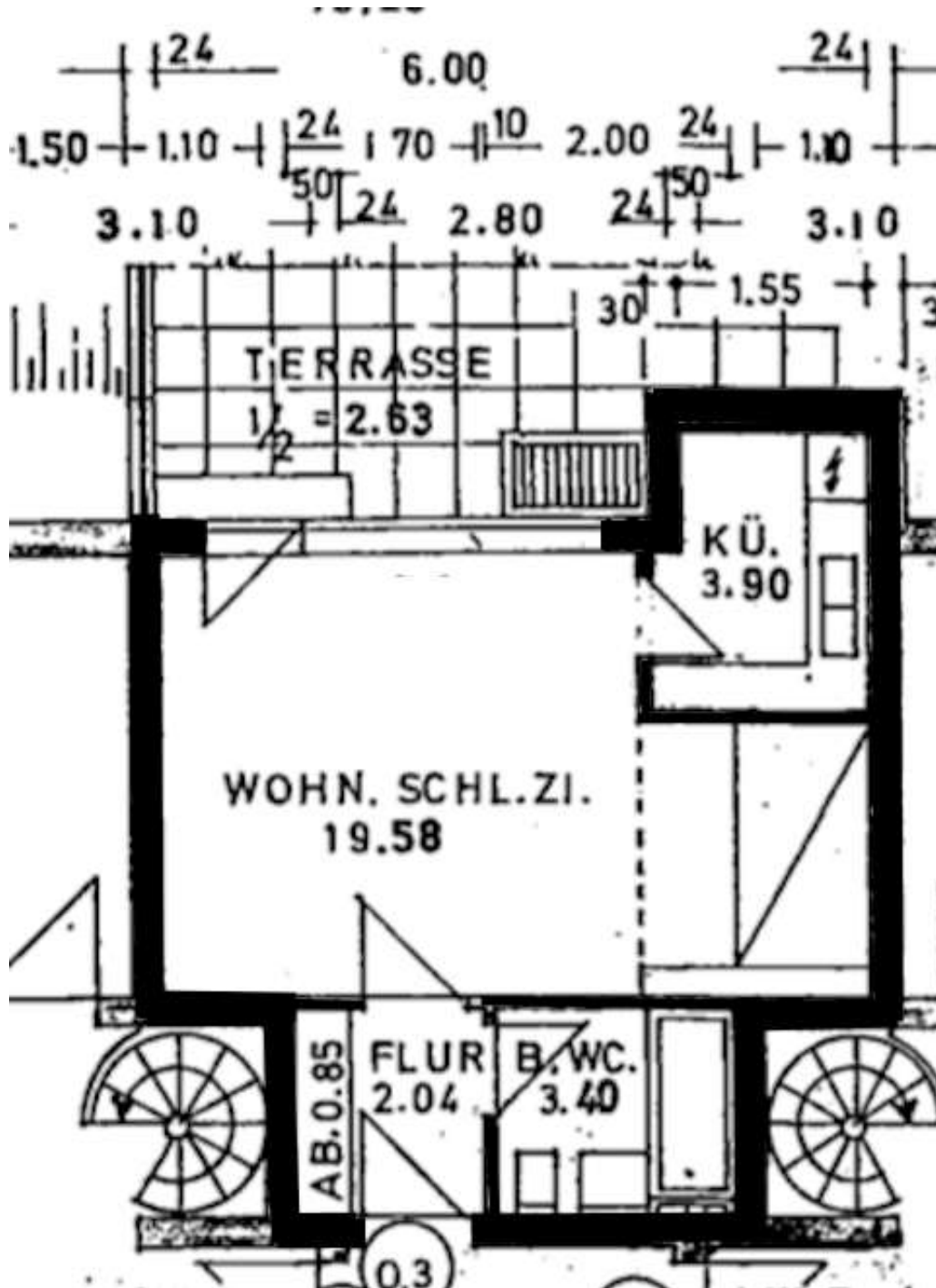
Grundriss Detail
